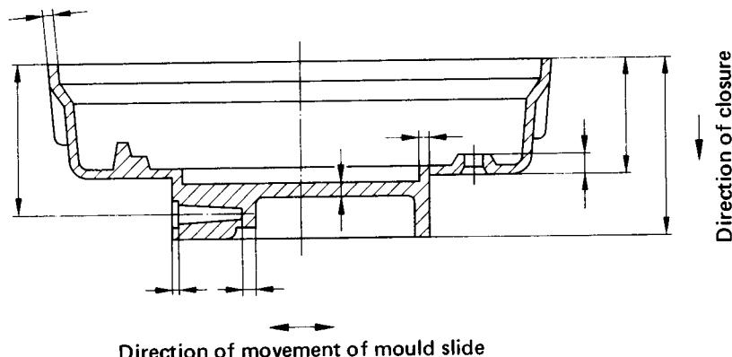
Figure 2. Non-mould-related dimensions
